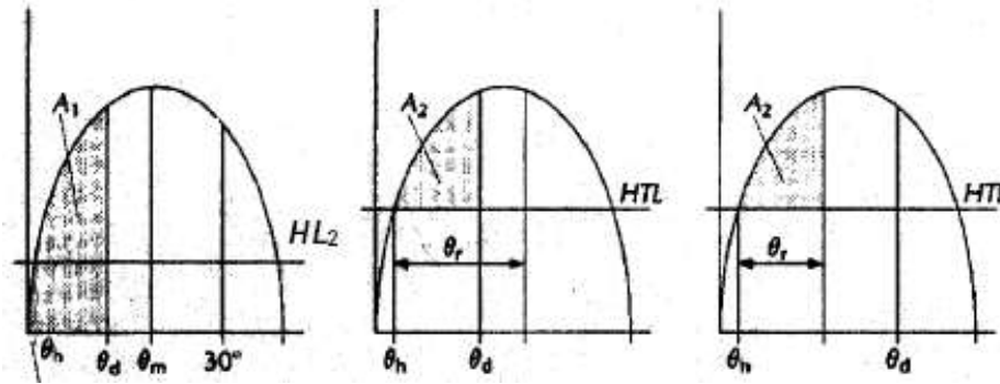
Figure 1 - Intact stability
